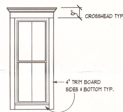
WINDOW TRIM DETAIL TYP.
