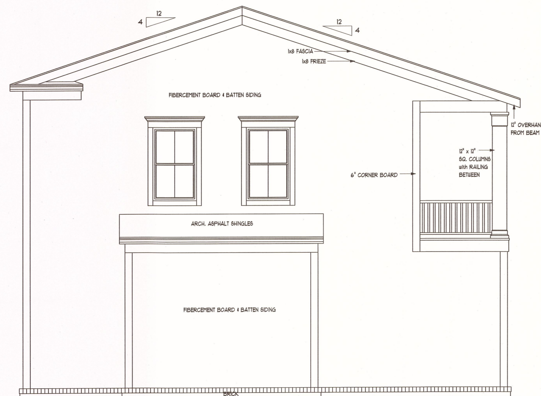
LEFT ELEVATION
