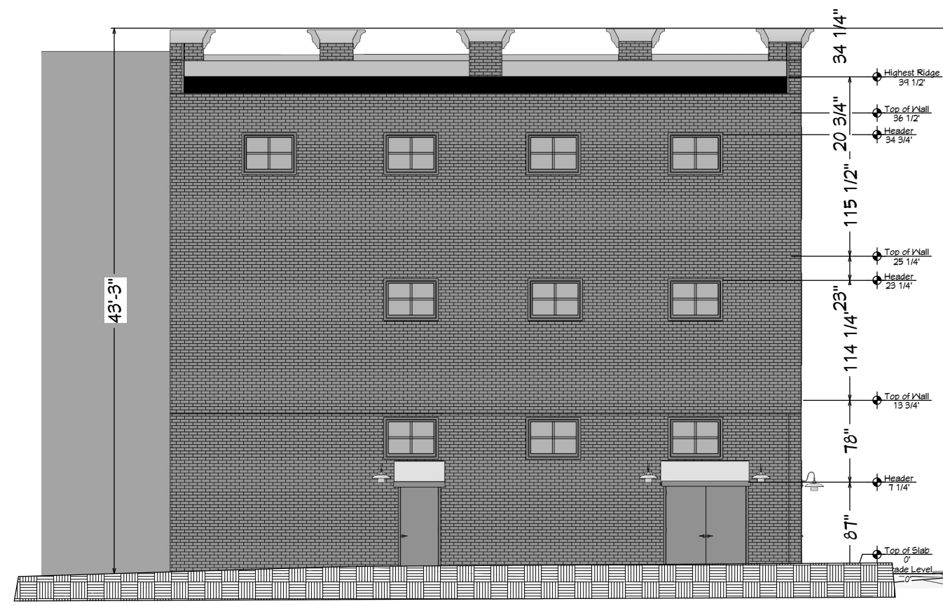
BACK ELEVATION
